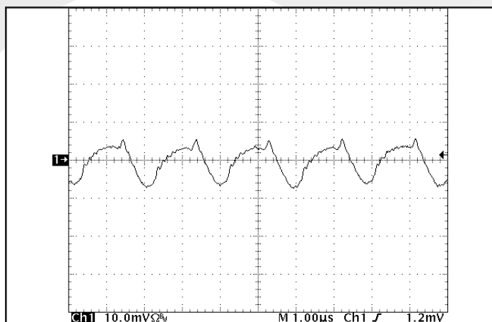
Figure 9: Input terminal current ripple, i_C , at full rated output current and nominal input voltage with 100 \mu H source impedance and 47 \mu F electrolytic capacitor (100mA/div). Bandwidth: 20MHz. Timescale: 1.00 \mu s/div. See Figure 17.
